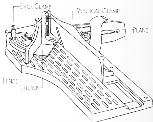
FIG. 213. MITER PLANE AND CHUTE BOARD.
